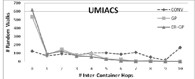
Figure 3. Histogram of Number of Inter-Container Hops for UMIACS Web Graph
