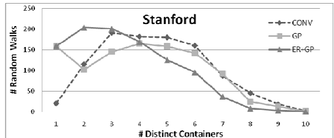
Figure 6. Histogram of Number of Distinct Containers Accessed for Stanford Web Graph
